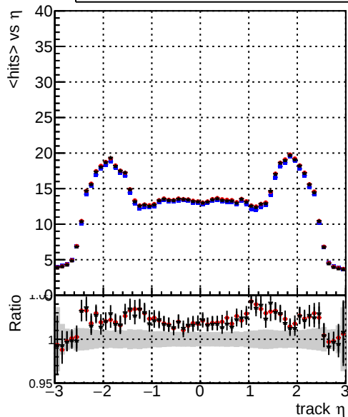
mean hit — DQM_original_step2_ttbar-phase1-newgeom — DQM_pixelCPETemplate_step2_ttbar-phase1-newgeom — DQM_pixelCPETemplateCutChiSquareNew5_step2_ttbar-phase1-newgeom
