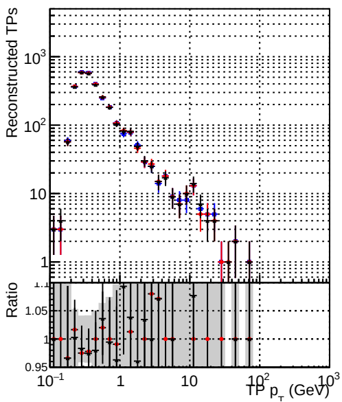
—•— DQM_original_step2_ttbar-phase1-newgeom —•— DQM_pixelCPETemplate_step2_ttbar-phase1-newgeom —•— DQM_pixelCPETemplateCutChiSquareNew5_step2_ttbar-phase1-newgeom
