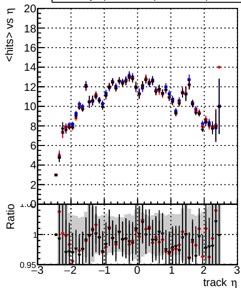
mean hits vs \eta — DQM_original_step2_ttbar-phase1-newgeom — DQM_pixelCPETemplate_step2_ttbar-phase1-newgeom — DQM_pixelCPETemplateCutChiSquareNew5_step2_ttbar-phase1-newgeom
