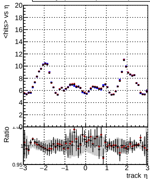
mean hits — DQM_original_step2_ttbar-phase1-newgeom — DQM_pixelCPETemplate_step2_ttbar-phase1-newgeom — DQM_pixelCPETemplateCutChiSquareNew5_step2_ttbar-phase1-newgeom
