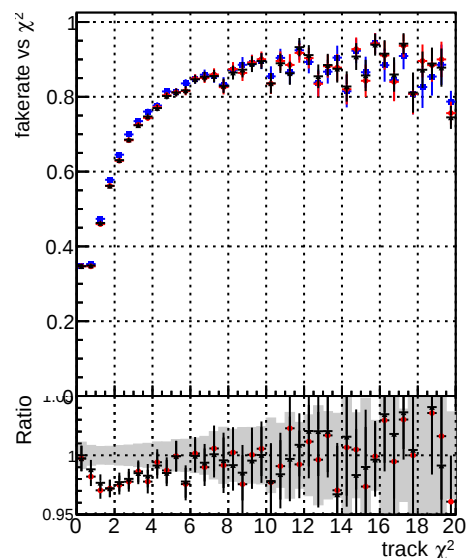
Fake rate vs. DOM original_step2_ttbare-phase1-newgeom DOM pixelfit_template_step2_ttbare-phase1-newgeom DOM pixelfit_template_step2_ttbare-phase1-newgeom
