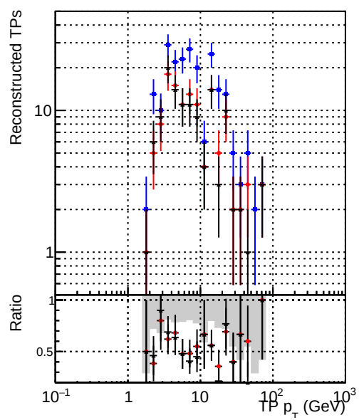
Legend: - DQM_original_step2_ttbar-phase1-newgeom (blue circles) - DQM_pixelCPETemplate_step2_ttbar-phase1-newgeom (red circles) - DQM_pixelCPETemplateCutChiSquareNew5_step2_ttbar-phase1-newgeom (black crosses)
