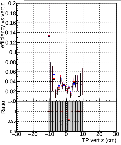
Efficiency vs TP vert z (cm) Legend: DQM_original_step2_ttbar-phase1-newgeom DQM_pixelCPETemplate_step2_ttbar-phase1-newgeom DQM_pixelCPETemplateCutChiSquareNew5_step2_ttbar-phase1-newgeom
