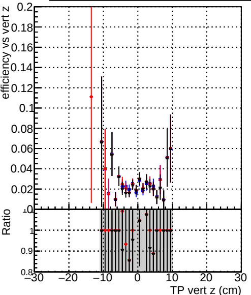
Efficiency vs TP vert z (cm) Legend: DQM_original_step2_ttbar-phase1-newgeom DQM_pixelCPETemplate_step2_ttbar-phase1-newgeom DQM_pixelCPETemplateCutChiSquareNew5_step2_ttbar-phase1-newgeom
