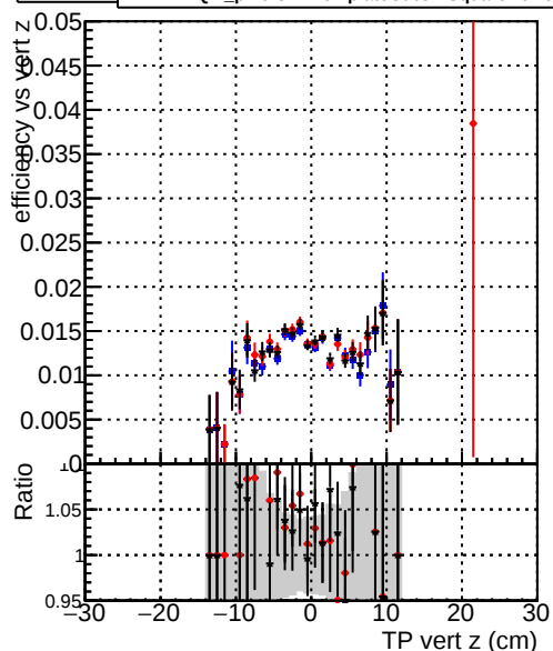
Efficiency vs. TP vert z — DQM_original_step2_ttbbar-phase1-newgeom — DQM_pixelCPETemplate_step2_ttbbar-phase1-newgeom — DQM_pixelCPETemplateCutChiSquareNew5_step2_ttbbar-phase1-newgeom
