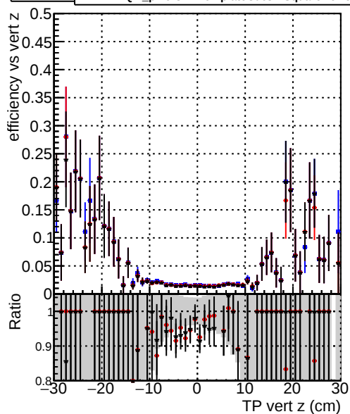
Efficiency vs vert z —•— DQM_original_step2_ttbar-phase1-newgeom —•— DQM_pixelCPETemplate_step2_ttbar-phase1-newgeom —•— DQM_pixelCPETemplateCutChiSquareNew5_step2_ttbar-phase1-newgeom
