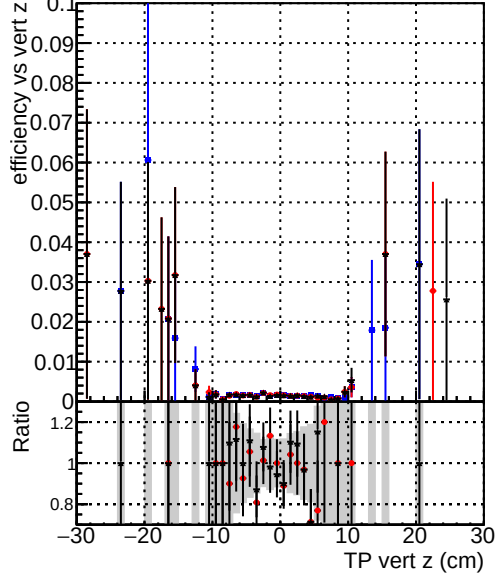
Efficiency vs. TP vert z —●— DQM_original_step2_ttbar-phase1-newgeom —●— DQM_pixelCPETemplate_step2_ttbar-phase1-newgeom —●— DQM_pixelCPETemplateCutChiSquareNew5_step2_ttbar-phase1-newgeom
