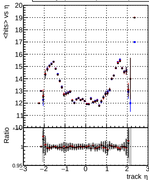
mean hits vs \eta — DQM_original_step2_ttbar-phase1-newgeom — DQM_pixelCPETemplate_step2_ttbar-phase1-newgeom — DQM_pixelCPETemplateCutChiSquareNew5_step2_ttbar-phase1-newgeom
