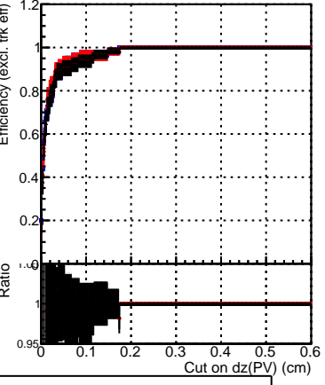
—■ DQM_original_step2_ttbar-phase1-newgeom —● DQM_pixelCPETemplate_step2_ttbar-phase1-newgeom —▲ DQM_pixelCPETemplateCutChiSquareNew5_step2_ttbar-phase1-newgeom
