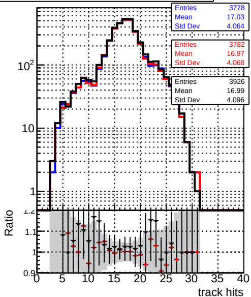
mean hits — DQM_original_step2_ttbar-phase1-newgeom — DQM_pixelCPETemplate_step2_ttbar-phase1-newgeom — DQM_pixelCPETemplateCutChiSquareNew5_step2_ttbar-phase1-newgeom
