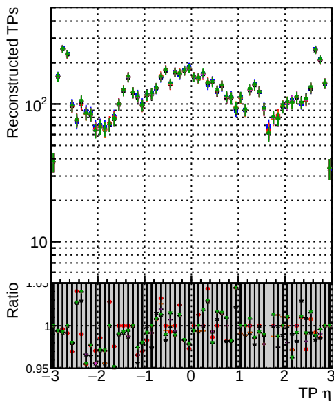
N of sim Model Pixel CPE Template Cut ChiSquare New2 Step2 ttbar phaset1 newgeom 1 DOM pixel CPE Template Cut ChiSquare New2 Step2 ttbar phaset1 newgeom 2 DOM pixel CPE Template Cut ChiSquare New3 Step2 ttbar phaset1 newgeom 3 DOM pixel CPE Template Cut ChiSquare New4 Step2 ttbar phaset1 newgeom
