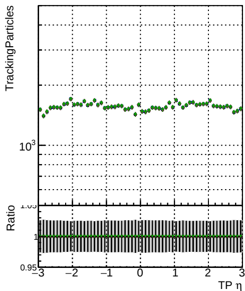
N of sim Model Pixel CPE Template Cut ChiSquare New2 Step2 ttbar phaset1 newgeom 1 DOM pixel CPE Template Cut ChiSquare New2 Step2 ttbar phaset1 newgeom 2 DOM pixel CPE Template Cut ChiSquare New3 Step2 ttbar phaset1 newgeom 3 DOM pixel CPE Template Cut ChiSquare New4 Step2 ttbar phaset1 newgeom
