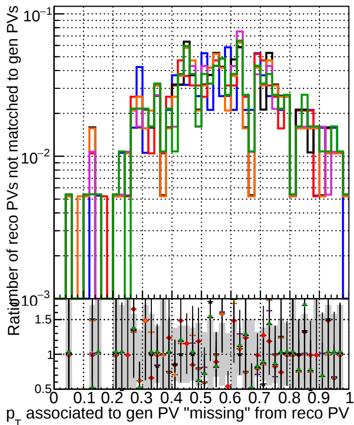
enew4_step2_lbar-phase1-newgeom recopvassoczgenfvnotmatched_missing
