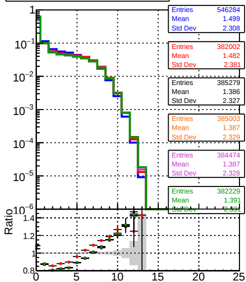
Legend: BOW, forward, step2, tbar, phase1-newgeom, BOW, pixel, CDD, TemplateCutChiSquareNew, step2, tbar, phase1-newgeom, BOW, pixel, CDD, TemplateCutChiSquareNew, step2, tbar, phase1-newgeom, BOW, pixel, CDD, TemplateCutChiSquareNew, step2, tbar, phase1-newgeom, BOW, pixel, CDD, TemplateCutChiSquareNew, step2, tbar, phase1-newgeom
