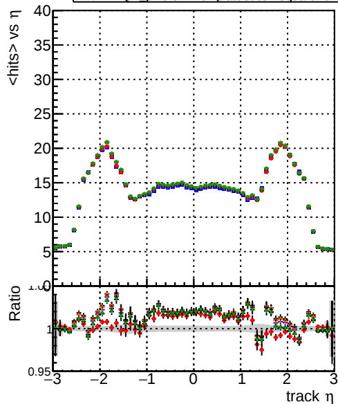
Legend: BOW, forward, step2, tbar, phase1-newgeom, BOW, pixel, CDD, TemplateCutChiSquareNew, step2, tbar, phase1-newgeom, BOW, pixel, CDD, TemplateCutChiSquareNew, step2, tbar, phase1-newgeom, BOW, pixel, CDD, TemplateCutChiSquareNew, step2, tbar, phase1-newgeom, BOW, pixel, CDD, TemplateCutChiSquareNew, step2, tbar, phase1-newgeom
