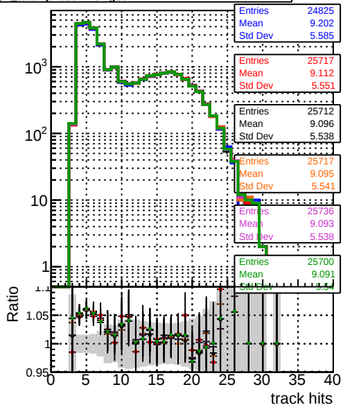
Legend: BDM, pixel, CDD, Template, CutCh, Square, New2, step2, tibar, phase1, newgeom mean hits
