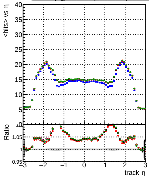
Legend: BOW, pixel, CDD, template, cutChiSquare, newgeom mean hits
