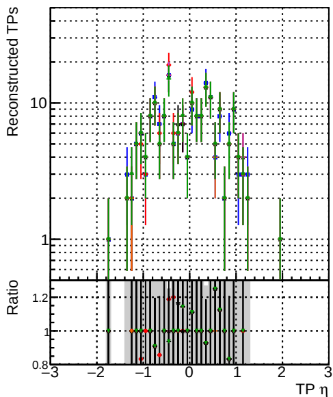
N of sim Model Pixel Template Cut ChiSquare New4 step2 tpar-phase1-newgeom 1 DOM pixel template Cut ChiSquare New4 step2 tpar-phase1-newgeom 2 DOM pixel template Cut ChiSquare New4 step2 tpar-phase1-newgeom 3 DOM pixel template Cut ChiSquare New4 step2 tpar-phase1-newgeom 4 DOM pixel template Cut ChiSquare New4 step2 tpar-phase1-newgeom
