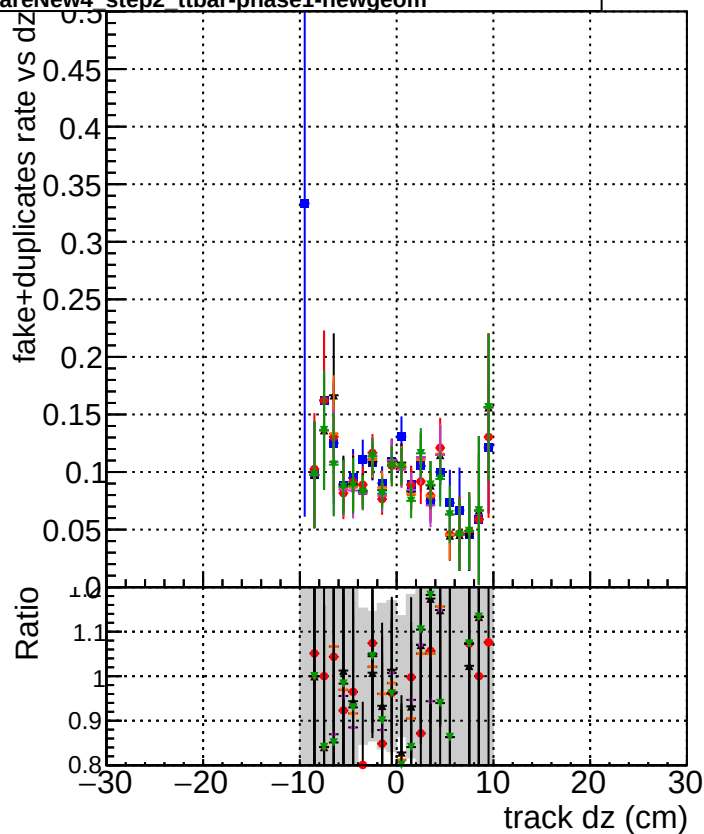
DOM original step2 ttbar-phase1-newgeom DOM pixelCPE1 template step2 ttbar-phase1-newgeom DOM pixelCPE1 templateCutChiSquareNew2 step2 ttbar-phase1-newgeom DOM pixelCPE1 templateCutChiSquareNew3 step2 ttbar-phase1-newgeom DOM pixelCPE1 templateCutChiSquareNew4 step2 ttbar-phase1-newgeom
