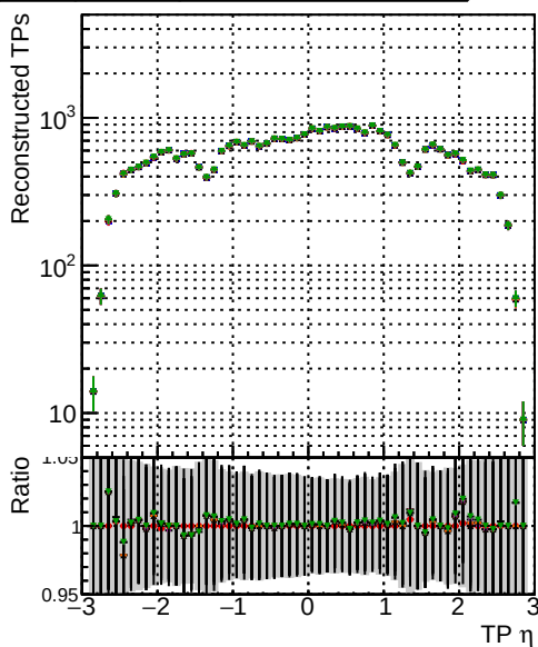
DOM original step2 thar-phase1-newgeom DOM pixe CPE template step2 thar-phase1-newgeom DOM pixe CPE template cutChiSquare new2 step2 thar-phase1-newgeom DOM pixe CPE template cutChiSquare new3 step2 thar-phase1-newgeom DOM pixe CPE template cutChiSquare new4 step2 thar-phase1-newgeom
