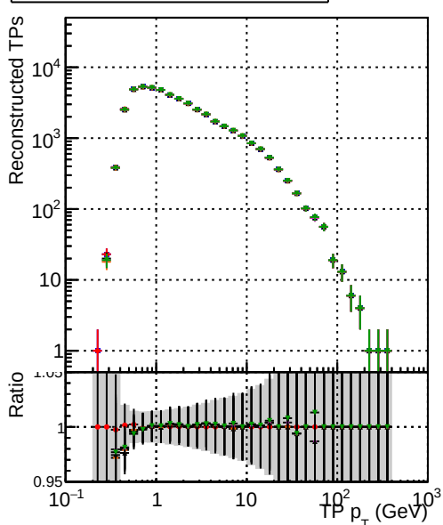
DOM original step2 thar-phase1-newgeom DOM pixe CPE template step2 thar-phase1-newgeom DOM pixe CPE template cutChiSquare new2 step2 thar-phase1-newgeom DOM pixe CPE template cutChiSquare new3 step2 thar-phase1-newgeom DOM pixe CPE template cutChiSquare new4 step2 thar-phase1-newgeom
