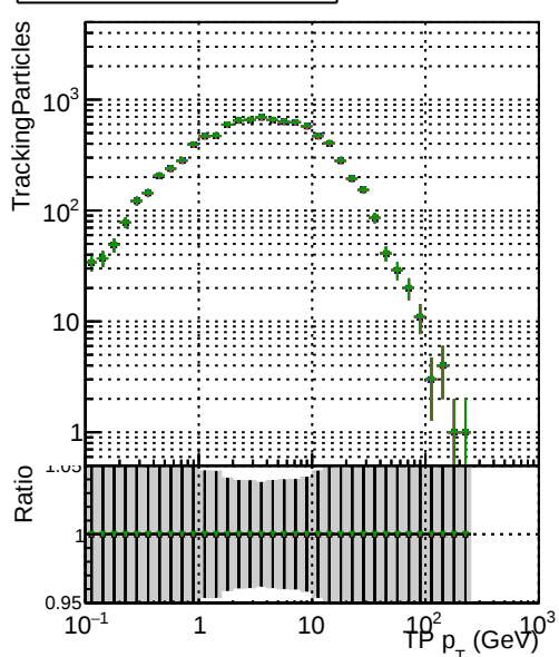
DOM original step2 ttar-phase1-newgeom DOM pixe CPE template step2 ttar-phase1-newgeom DOM pixe CPE template cutChiSquare new2 step2 ttar-phase1-newgeom DOM pixe CPE template cutChiSquare new3 step2 ttar-phase1-newgeom DOM pixe CPE template cutChiSquare new4 step2 ttar-phase1-newgeom
