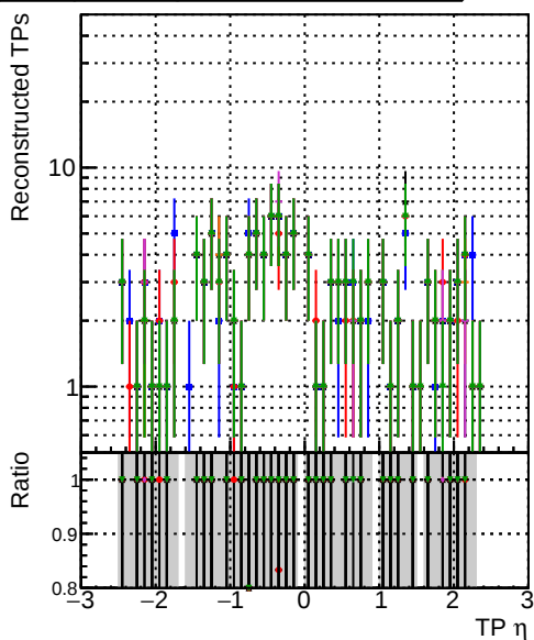
DOM original step2 ttar-phase1-newgeom DOM pixe CPE template step2 ttar-phase1-newgeom DOM pixe CPE template cutChiSquare new2 step2 ttar-phase1-newgeom DOM pixe CPE template cutChiSquare new3 step2 ttar-phase1-newgeom DOM pixe CPE template cutChiSquare new4 step2 ttar-phase1-newgeom
