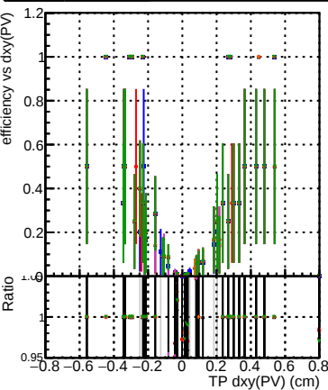
Efficiency vs Dxy(PV) (cm) Legend: DOM original_step2_ttbar-phase1-newgeom DOM pixelCPETemplate_step2_ttbar-phase1-newgeom DOM pixelCPETemplateCutChiSquareNew_step2_ttbar-phase1-newgeom DOM pixelCPETemplateCutChiSquareNew2_step2_ttbar-phase1-newgeom DOM pixelCPETemplateCutChiSquareNew3_step2_ttbar-phase1-newgeom DOM pixelCPETemplateCutChiSquareNew4_step2_ttbar-phase1-newgeom
