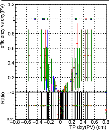
Efficiency vs Dxy(PV) (cm) Legend: DOM original step2 ttbar-phase1-newgeom DOM pixelCPTemplate step2 ttbar-phase1-newgeom DOM pixelCPTemplateCutChiSquareNew step2 ttbar-phase1-newgeom DOM pixelCPTemplateCutChiSquareNew2 step2 ttbar-phase1-newgeom DOM pixelCPTemplateCutChiSquareNew3 step2 ttbar-phase1-newgeom DOM pixelCPTemplateCutChiSquareNew4 step2 ttbar-phase1-newgeom
