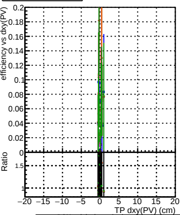
Efficiency vs Dxy(PV) (cm) Legend: DOM original step2 ttbar-phase1-newgeom DOM pixelCPTemplate step2 ttbar-phase1-newgeom DOM pixelCPTemplateCutChiSquareNew step2 ttbar-phase1-newgeom DOM pixelCPTemplateCutChiSquareNew2 step2 ttbar-phase1-newgeom DOM pixelCPTemplateCutChiSquareNew3 step2 ttbar-phase1-newgeom DOM pixelCPTemplateCutChiSquareNew4 step2 ttbar-phase1-newgeom
