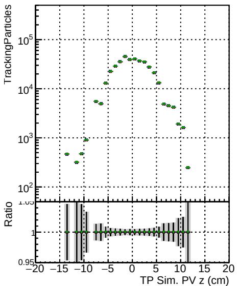
N of simulated tracks vs. sim PV z 10000 1000 100 10 1
