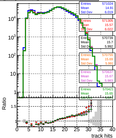
Legend: BOW original, step2, tbar, phase1-newgeom, BOW pixel, CDD, TemplateCutChiSquareNew4, BOW pixel, CDD, TemplateCutChiSquareNew2, BOW pixel, CDD, TemplateCutChiSquareNew1, BOW pixel, CDD, TemplateCutChiSquareNew4
