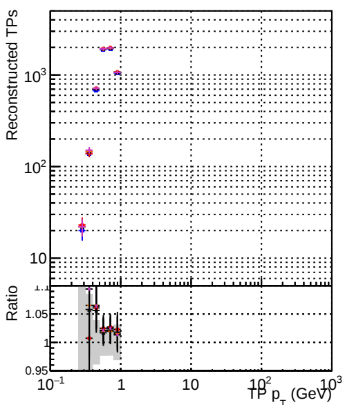
— DOM original step2 ttbar-phase1-newgeom — DOM pixelCPETemplateCut step2 ttbar-phase1-newgeom — DOM pixelCPETemplateCutChiSquareNew step2 ttbar-phase1-newgeom — DOM pixelCPETemplateCutChiSquareNew2 step2 ttbar-phase1-newgeom — DOM pixelCPETemplateCutChiSquareNew3 step2 ttbar-phase1-newgeom
