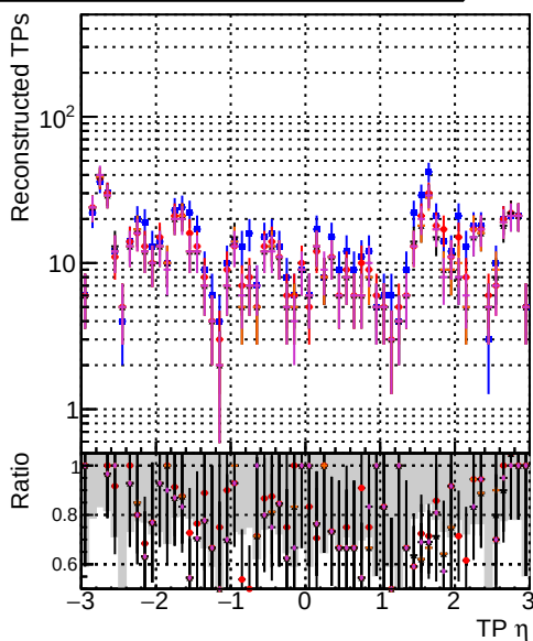
—•— DQM original step2 ttbar-phase1-newgeom —•— DQM pixelCPETemplateCutChiSquareNew step2 ttbar-phase1-newgeom —•— DQM pixelCPETemplateCutChiSquareNew2 step2 ttbar-phase1-newgeom —•— DQM pixelCPETemplateCutChiSquareNew3 step2 ttbar-phase1-newgeom
