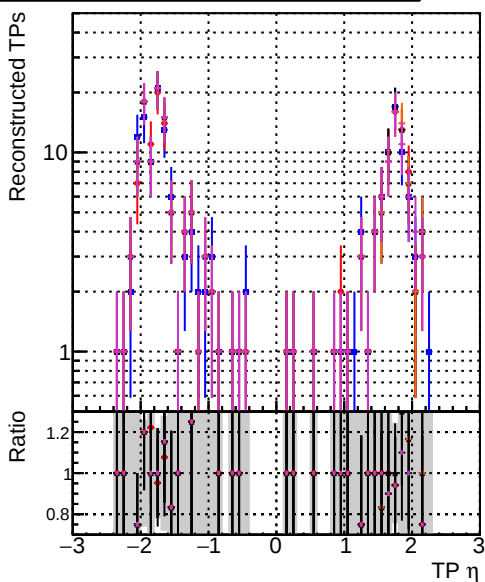
—•— DOM original step2 ttbar-phase1-newgeom —•— DOM pixelCPETemplateCutChiSquareNew step2 ttbar-phase1-newgeom —•— DOM pixelCPETemplateCutChiSquareNew2 step2 ttbar-phase1-newgeom —•— DOM pixelCPETemplateCutChiSquareNew3 step2 ttbar-phase1-newgeom
