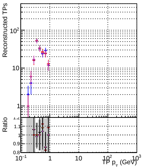
—•— DOM original step2 ttbar-phase1-newgeom —•— DOM pixelCPETemplateCutChiSquareNew step2 ttbar-phase1-newgeom —•— DOM pixelCPETemplateCutChiSquareNew2 step2 ttbar-phase1-newgeom —•— DOM pixelCPETemplateCutChiSquareNew3 step2 ttbar-phase1-newgeom
