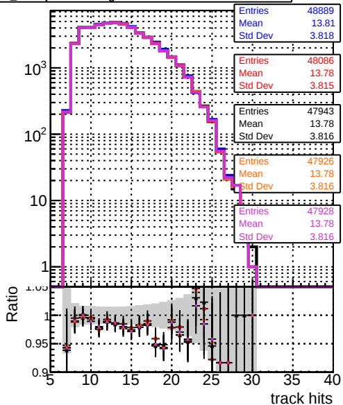
DOM original step2 ttbar-phase1-newgeom DOM pixeICPETemplate step2 ttbar-phase1-newgeom DOM pixeICPETemplateCutChiSquareNew step2 ttbar-phase1-newgeom DOM pixeICPETemplateCutChiSquareNew3 step2 ttbar-phase1-newgeom
