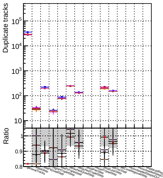
DOM pixelCPEtemplateCutChiSquareNew step2 ttbar-phase1-newgeom Number DOM pixelCPEtemplateCutChiSquareNew2 step2 ttbar-phase1-newgeom DOM pixelCPEtemplateCutChiSquareNew3 step2 ttbar-phase1-newgeom DOM pixelCPEtemplateCutChiSquareNew3 step2 ttbar-phase1-newgeom
