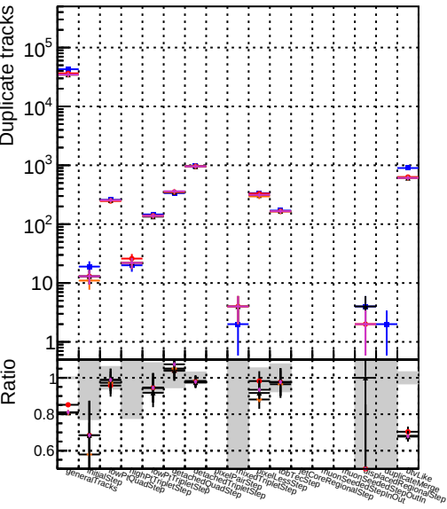
Number Diagram Label 1 DQM pixelCPETemplateCutChiSquareNew_step2_ttbar-phase1-newgeom 2 DQM pixelCPETemplateCutChiSquareNew2_step2_ttbar-phase1-newgeom 3 DQM pixelCPETemplateCutChiSquareNew3_step2_ttbar-phase1-newgeom
