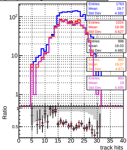
DQM original step2 ttbar-phase1-newgeom DQM pixelCPETemplateCutChiSquareNew3 step2 ttbar-phase1-newgeom DQM pixelCPETemplateCutChiSquareNew2 step2 ttbar-phase1-newgeom DQM pixelCPETemplateCutChiSquareNew1 step2 ttbar-phase1-newgeom
