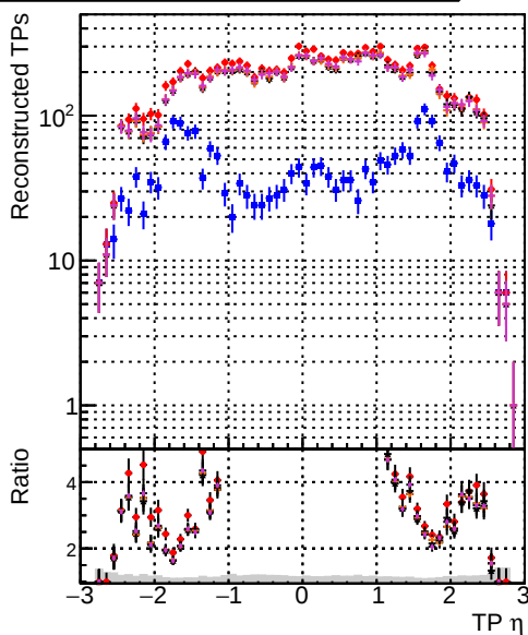
— DOM original step2 tbar-phase1-newgeom — DOM pixelCPETemplate step2 tbar-phase1-newgeom — DOM pixelCPETemplateCutChiSquareNew step2 tbar-phase1-newgeom — DOM pixelCPETemplateCutChiSquareNew2 step2 tbar-phase1-newgeom — DOM pixelCPETemplateCutChiSquareNew3 step2 tbar-phase1-newgeom
