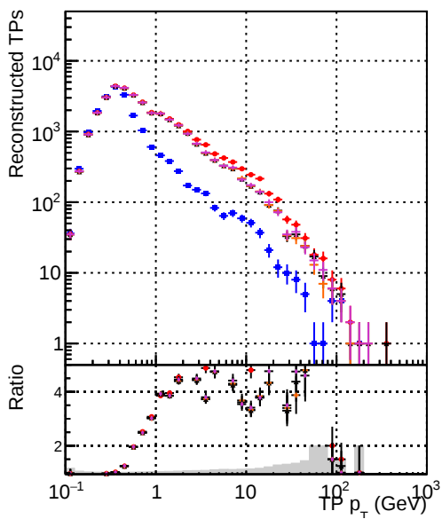
— DOM original step2 tbar-phase1-newgeom — DOM pixelCPETemplate step2 tbar-phase1-newgeom — DOM pixelCPETemplateCutChiSquareNew step2 tbar-phase1-newgeom — DOM pixelCPETemplateCutChiSquareNew2 step2 tbar-phase1-newgeom — DOM pixelCPETemplateCutChiSquareNew3 step2 tbar-phase1-newgeom
