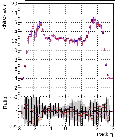
Legend for mean hits vs \eta : DOM original step2 ttbar-phase1-newgeom DOM pixelCPETemplate step2 ttbar-phase1-newgeom DOM pixelCPETemplateCutChiSquareNew step2 ttbar-phase1-newgeom DOM pixelCPETemplateCutChiSquareNew2 step2 ttbar-phase1-newgeom DOM pixelCPETemplateCutChiSquareNew3 step2 ttbar-phase1-newgeom
