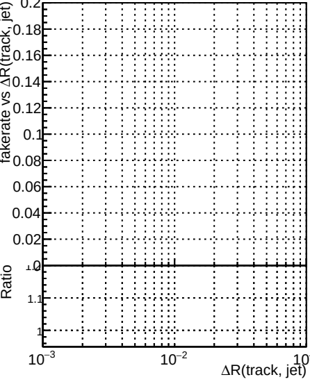
Fake rate vs \Delta R(\text{track, jet}) DQM original_step2_tbar_phase1_newgeom DQM+DPM DQM+DPM+template DQM+DPM+template+chi2square New3_step2_tbar_phase1_newgeom DQM+DPM+template+chi2square+New3_step2_tbar_phase1_newgeom
