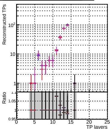
2_ttbar-phase1-newgeom 2_ttbar-phase1-newgeom
