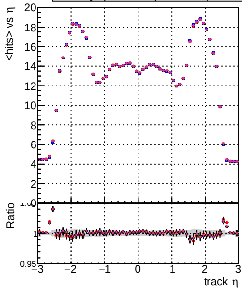
DOM original step2 ttbar-phase1-newgeom DOM pixelCPETemplate step2 ttbar-phase1-newgeom DOM pixelCPETemplateCutChiSquareNew step2 ttbar-phase1-newgeom DOM pixelCPETemplateCutChiSquareNew2 step2 ttbar-phase1-newgeom DOM pixelCPETemplateCutChiSquareNew3 step2 ttbar-phase1-newgeom
