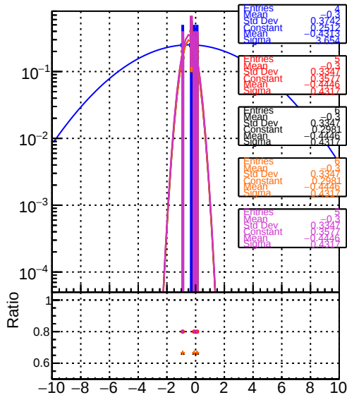
DOM original step2 tthar phase1 newgeom
