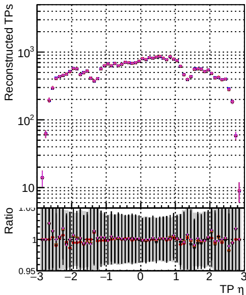
— DOM original step2 ttbar-phase1-newgeom — DOM pixelCPETemplate step2 ttbar-phase1-newgeom — DOM pixelCPETemplateCutChiSquareNew step2 ttbar-phase1-newgeom — DOM pixelCPETemplateCutChiSquareNew3 step2 ttbar-phase1-newgeom
