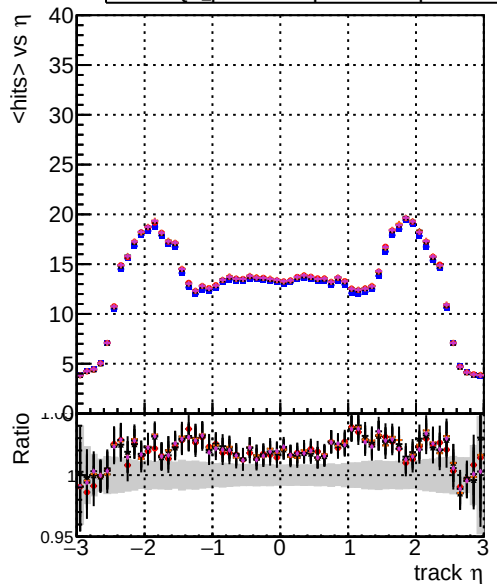
DOM original step2 ttbar-phase1-newgeom DOM pixeICPETemplate step2 ttbar-phase1-newgeom DOM pixeICPETemplateCutChiSquareNew step2 ttbar-phase1-newgeom DOM pixeICPETemplateCutChiSquareNew2 step2 ttbar-phase1-newgeom DOM pixeICPETemplateCutChiSquareNew3 step2 ttbar-phase1-newgeom
