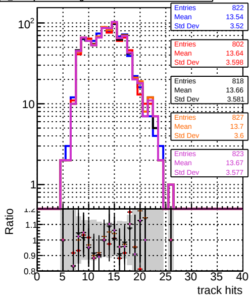
mean hits DOM original step2 ttbar-phase1-newgeom DOM pixeICPETemplate step2 ttbar-phase1-newgeom DOM pixeICPETemplateCutChiSquareNew step2 ttbar-phase1-newgeom DOM pixeICPETemplateCutChiSquareNew3 step2 ttbar-phase1-newgeom
