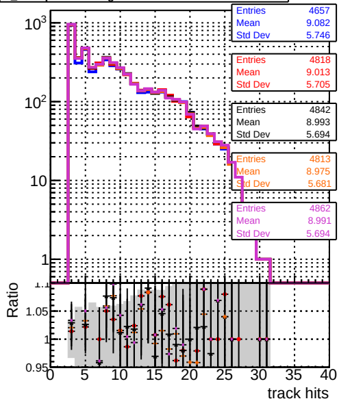
mean hit DOM original step2 ttbar-phase1-newgeom DOM pixelCPETemplate step2 ttbar-phase1-newgeom DOM pixelCPETemplateCutChiSquareNew2 step2 ttbar-phase1-newgeom DOM pixelCPETemplateCutChiSquareNew3 step2 ttbar-phase1-newgeom
