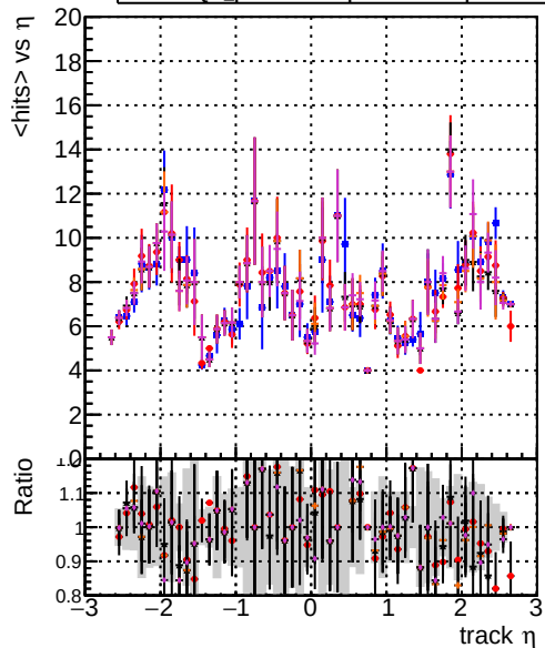
DQM-original-step2-ttbar-phase1-newgeom DQM-pixelCPE-template-step2-ttbar-phase1-newgeom DQM-pixelCPE-template-cut-chi-square-new3-step2-ttbar-phase1-newgeom DQM-pixelCPE-template-cut-chi-square-new2-step2-ttbar-phase1-newgeom DQM-pixelCPE-template-cut-chi-square-new3-step2-ttbar-phase1-newgeom
