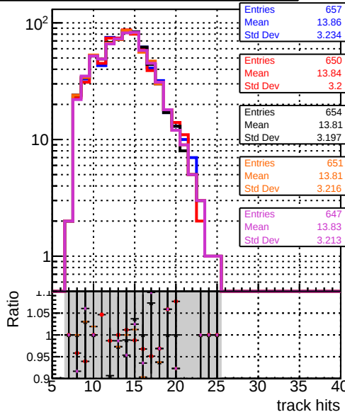
mean hit DQM original step2 ttbar-phase1-newgeom DQM pixelCPETemplate step2 ttbar-phase1-newgeom DQM pixelCPETemplateCutChiSquareNew2 step2 ttbar-phase1-newgeom DQM pixelCPETemplateCutChiSquareNew3 step2 ttbar-phase1-newgeom
