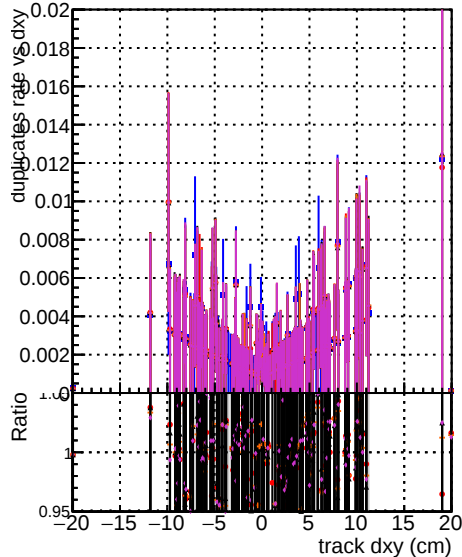
SquareNew3-step2-ttbar-phase1-newgeom
