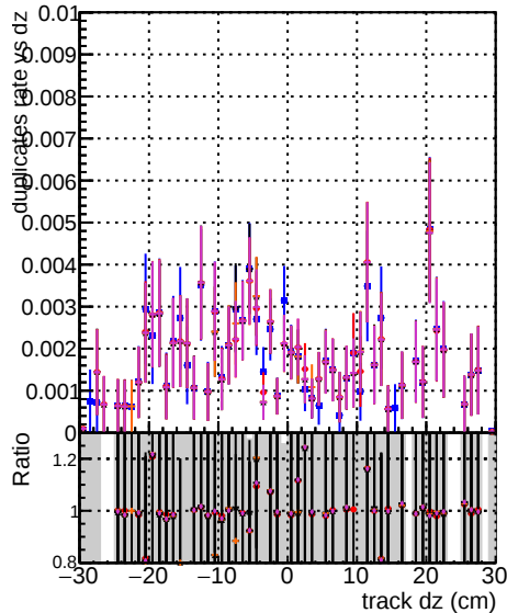
SquareNew3-step2-ttbar-phase1-newgeom
