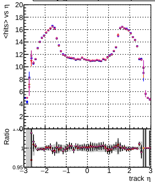
DOM original step2 ttbar-phase1-newgeom DOM pixelCPETemplate step2 ttbar-phase1-newgeom DOM pixelCPETemplateCutChiSquareNew step2 ttbar-phase1-newgeom DOM pixelCPETemplateCutChiSquareNew3 step2 ttbar-phase1-newgeom
