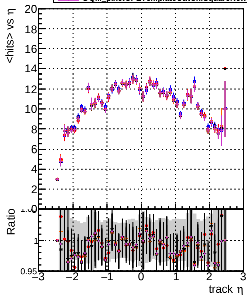
DOM original step2 ttbar-phase1-newgeom DOM pixelCPETemplate step2 ttbar-phase1-newgeom DOM pixelCPETemplateCutChiSquareNew step2 ttbar-phase1-newgeom DOM pixelCPETemplateCutChiSquareNew3 step2 ttbar-phase1-newgeom
