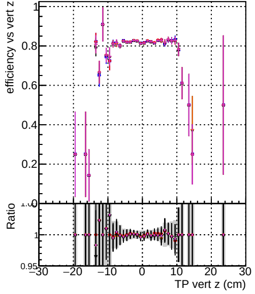
— DOM original step2 ttbar-phase1-newgeom — pixelCPE Template step2 ttbar-phase1-newgeom — pixelCPE TemplateCutChiSquareNew3 step2 ttbar-phase1-newgeom — pixelCPE TemplateCutChiSquareNew2 step2 ttbar-phase1-newgeom — pixelCPE TemplateCutChiSquareNew3 step2 ttbar-phase1-newgeom
